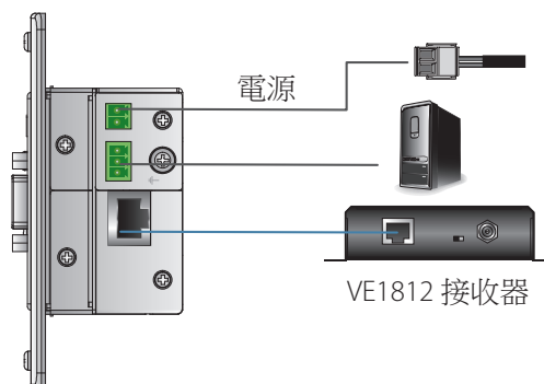
VE2812UST (側視圖)
